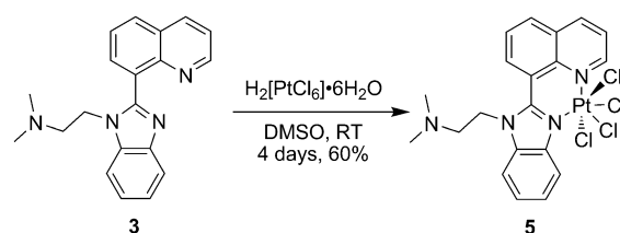
Scheme 3. Synthesis of [Pt IV (N,N-dimethyl-2-[2-(quinolin-8-yl)-1H-benzimidazol-1-yl]ethanamine)Cl 4 ] (5).
