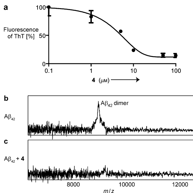
Figure 1. Inhibition of \text{A}\beta aggregation. a) Fluorescence emission spectra of thioflavin T (ThT) upon addition of \text{A}\beta_{42} ( 10 \mu\text{M} ) incubated with 4 in various concentrations at RT for 24 h. Inhibition of \text{A}\beta amyloid formation by 4 was observed in a dose-dependent manner. Error bars: \pm standard deviation. b, c) SELDI-TOF mass spectrum of \text{A}\beta_{42} ( 10 \mu\text{M} ) incubated b) with vehicle at RT for 6 h to show the formation of dimeric \text{A}\beta_{42} , and c) with 4 ( 10 \mu\text{M} ) at RT for 6 h, showing that the dimeric form of \text{A}\beta is absent.
